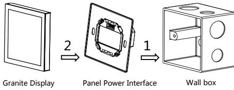
Figure 5. Installation
